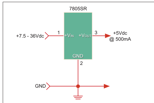
Figure 1. Typical Connections
