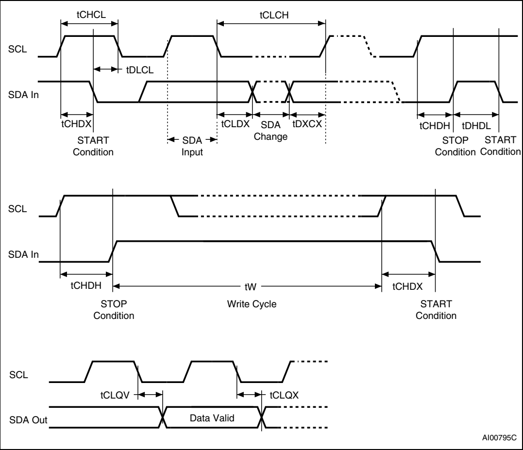
Figure 13. AC waveforms
