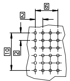
LAYOUT FOR P.C.B (PER 12mm LENGTH)
