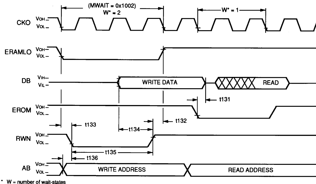
Figure 17. External Memory Data Write Timing Diagram
