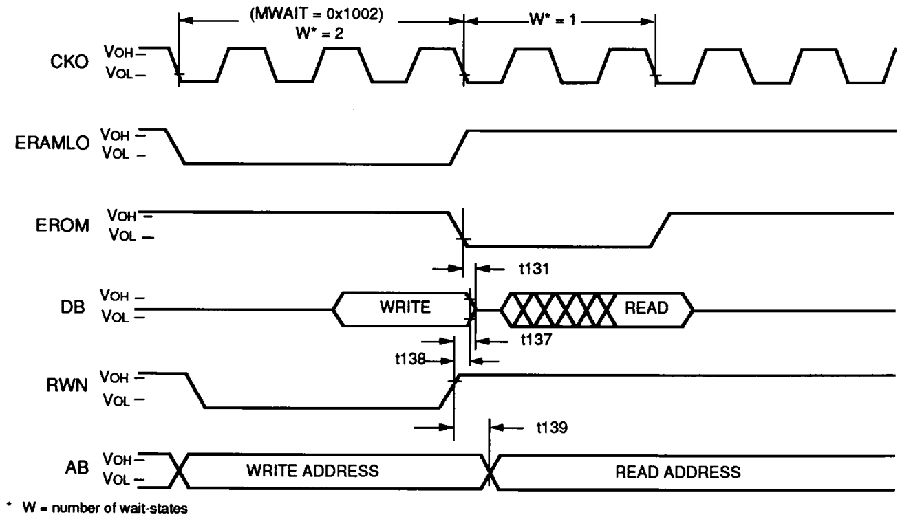
Figure 18. Write Cycle Followed by Read Cycle
