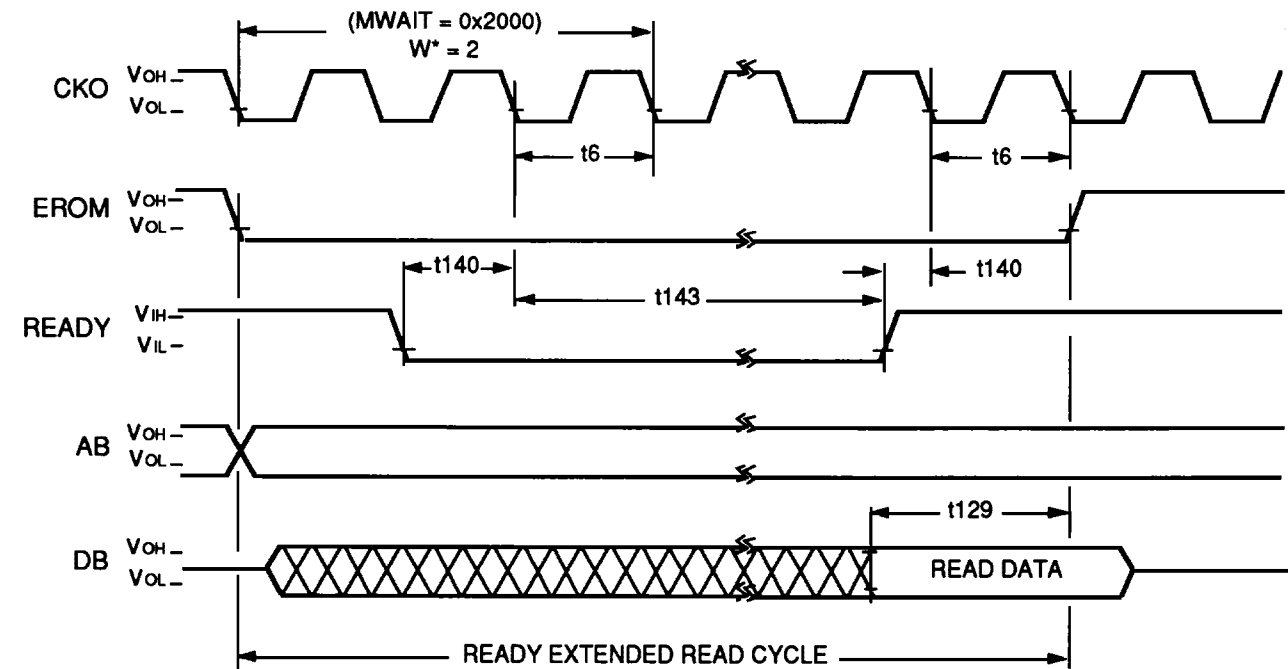
Figure 19. READY† Extended Read Cycle Timing
