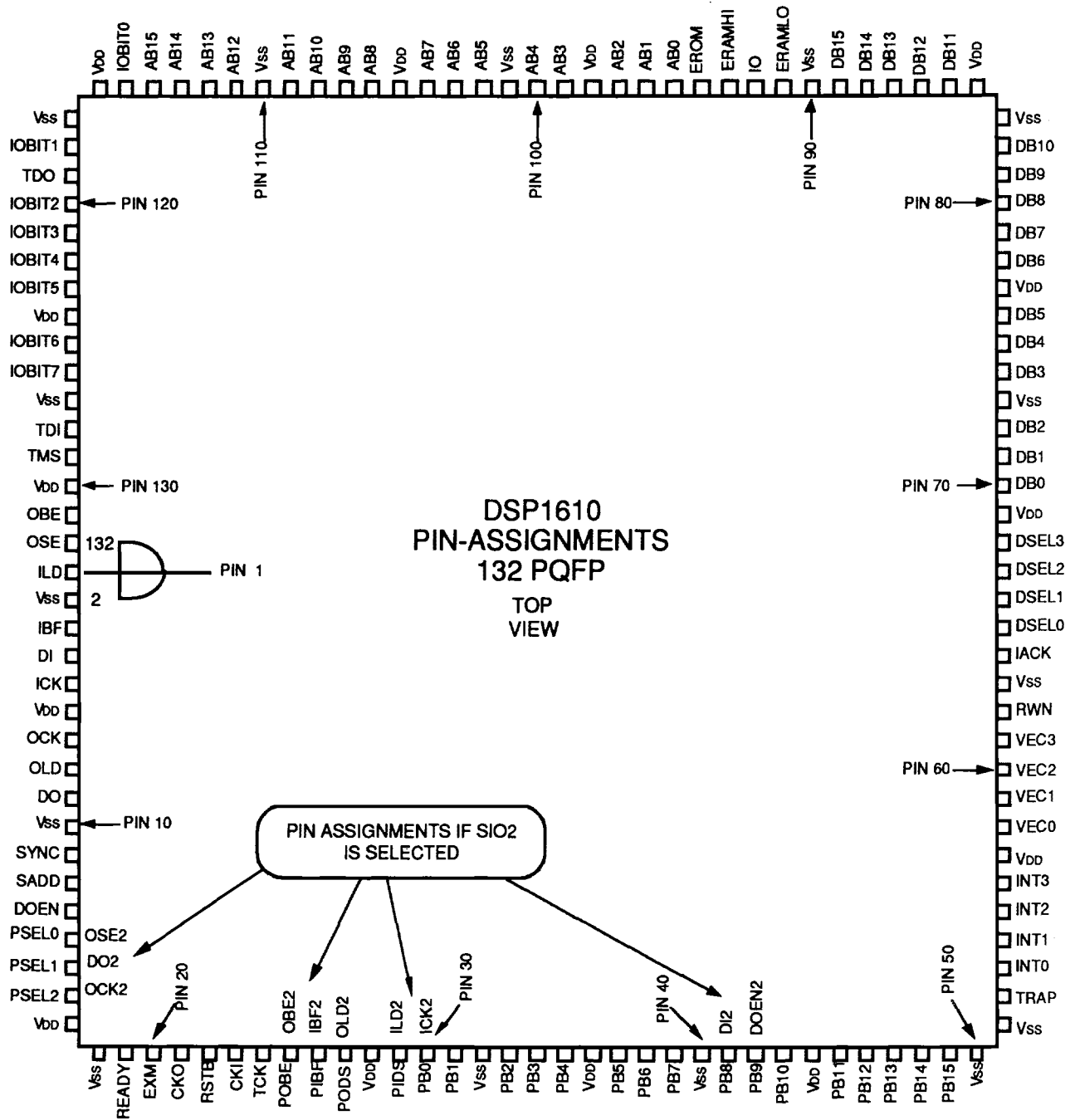
Figure 1. Pin Diagram
