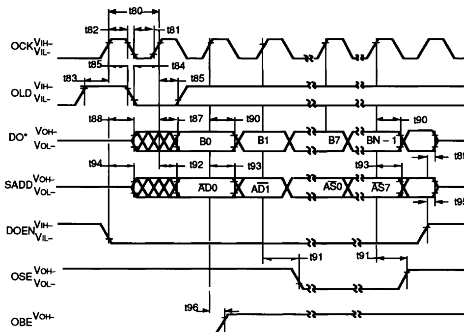
Figure 28. SIO Passive Mode Output Timing Diagram
