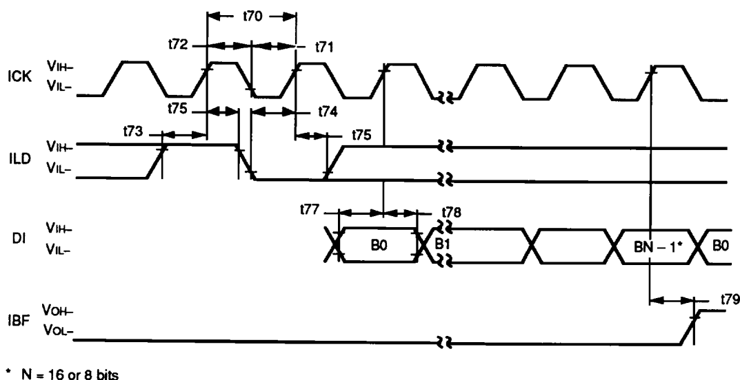
Figure 26. SIO Passive Mode Input Timing Diagram
