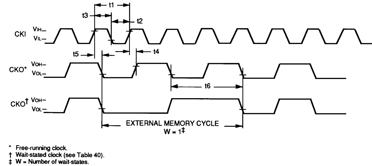
Figure 8. I/O Clock Timing Diagram
