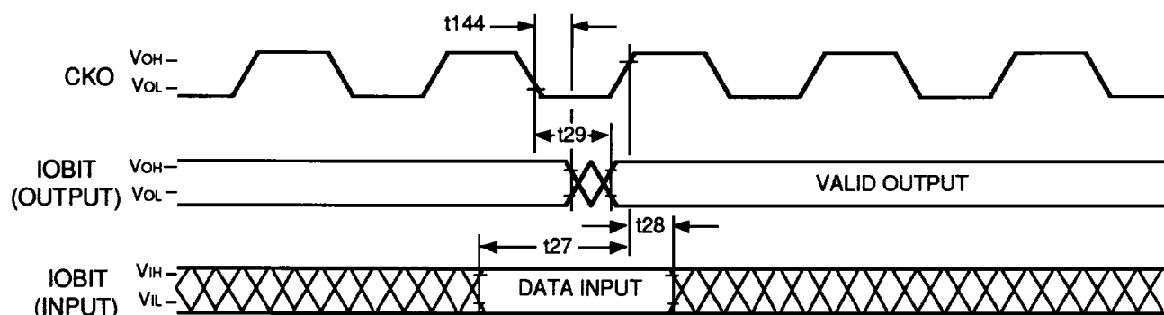
Figure 13. Write Outputs Followed by Read Inputs (cbit = Immediate a1 = sb1t)
