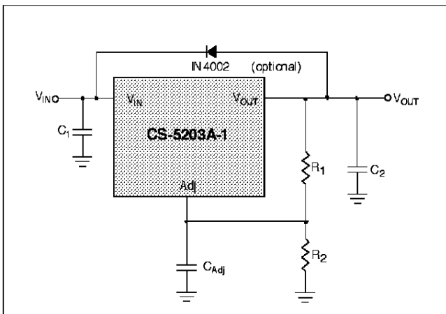
Figure 2a. Protection diode scheme for adjustable output regulator.
