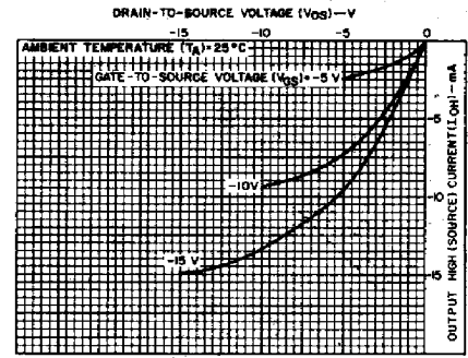
Fig. 9 — Minimum p-channel output high (source) current characteristics.
