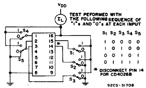
Fig. 15 - Quiescent device current.
