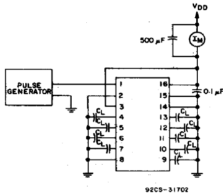
Fig. 14 - Dynamic power dissipation test circuit for CD4033B.
