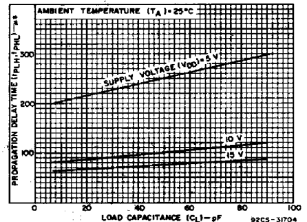
Fig. 11 — Typical propagation delay time as a function of load capacitance for carry-out outputs.
