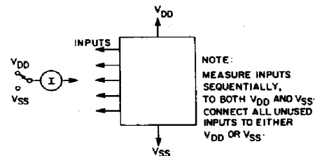
Fig. 17 - Input current.
