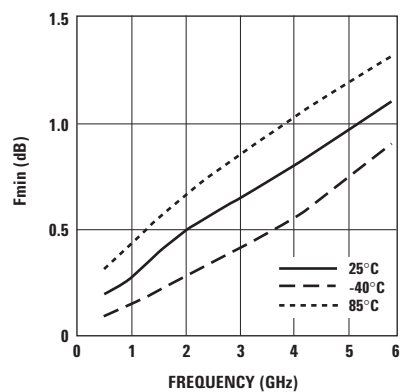
Figure 15. Fmin vs. Frequency and Temp. Tuned for Max OIP3 and Fmin at 3V, 30 mA.
