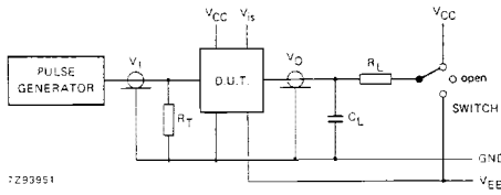
Fig. 20 Test circuit for measuring AC performance.
