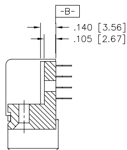
SECTION C-C
