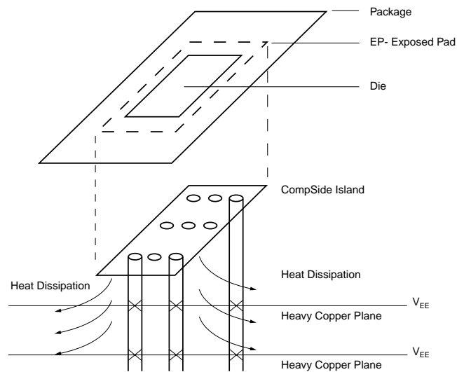
PCB Thermal Consideration for 28-Pin EPAD-SOIC Package
