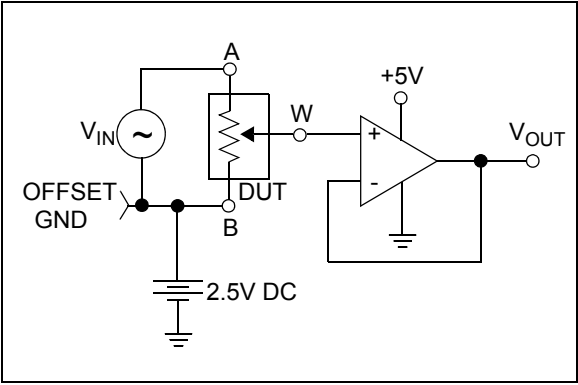
FIGURE 2-49: Gain vs. Frequency (-3 dB Bandwidth) Test Circuit.
