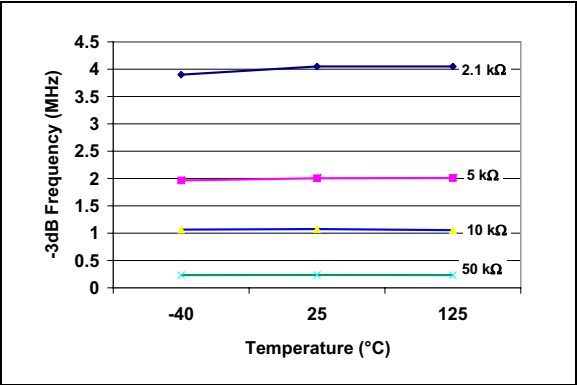
FIGURE 2-48: Gain vs. Frequency (-3 dB Bandwidth).
