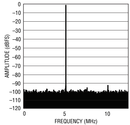
LTC2170-12: 8k Point FFT, f_{IN} = 70\text{MHz}, -1\text{dBFS}, 25\text{Msps}
