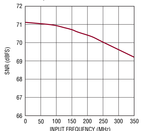
LTC2172-12: SNR vs Input Frequency, -1\text{dBFS} , 2\text{V Range} , 65\text{Mpsps}
