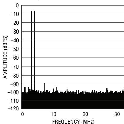
LTC2172-12: 8k Point 2-Tone FFT, f_{IN} = 68\text{MHz} , 69\text{MHz} , -1\text{dBFS} , 65\text{Mpsps}
