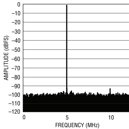
LTC2170-12: 8k Point FFT, f_{IN} = 30\text{MHz}, -1\text{dBFS}, 25\text{Msps}
