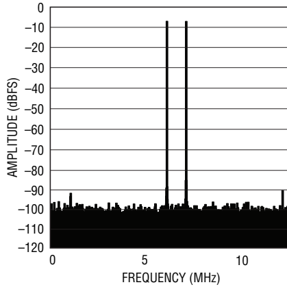
LTC2170-12: 8k Point 2-Tone FFT, f_{IN} = 68\text{MHz}, 69\text{MHz}, -1\text{dBFS}, 25\text{Msps}
