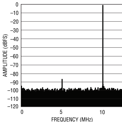
LTC2170-12: 8k Point FFT, f_{IN} = 140\text{MHz}, -1\text{dBFS}, 25\text{Msps}
