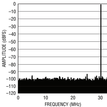
LTC2172-12: 8k Point FFT, f_{IN} = 30\text{MHz} , -1\text{dBFS} , 65\text{Mpsps}
