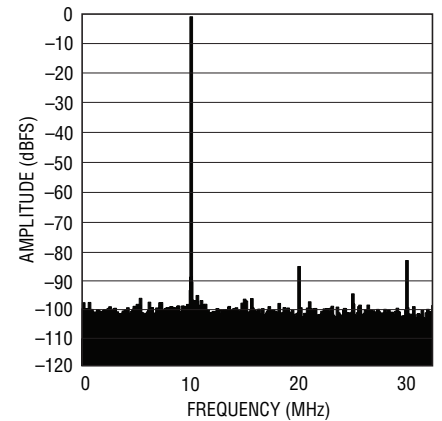
LTC2172-12: 8k Point FFT, f_{IN} = 140\text{MHz} , -1\text{dBFS} , 65\text{Mpsps}
