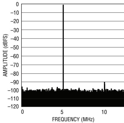
LTC2170-12: 8k Point FFT, f_{IN} = 5\text{MHz}, -1\text{dBFS}, 25\text{Msps}
