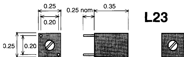
Standard small footprint vertical adjust version
