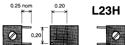
Optional low profile horizontal adjust version
