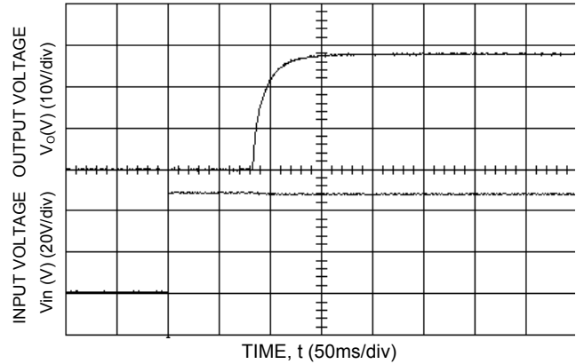
Figure 5. Typical Start-Up Using from V IN , positive logic version shown; C o,ext = 470µF.
