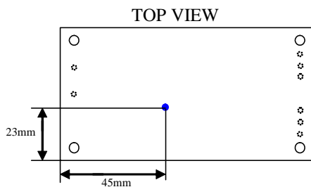
Figure 14. Case ( T_c ) Temperature Measurement Location (top view).
