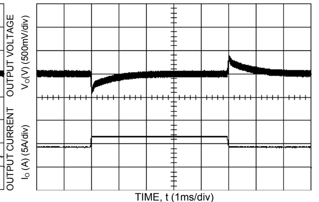
Figure 6. Transient Response to Dynamic Load Change from 50% to 75% to 50% of Full Load at Room Temperature and 48 Vdc Input; 0.1A/uS
