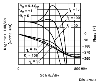
Frequency Response for Various R_L S
