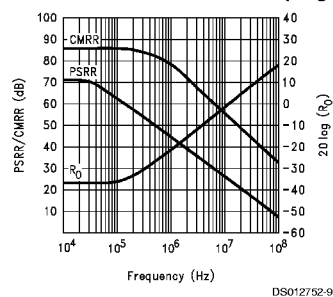
PSRR, CMRR, and Closed Loop R_O
