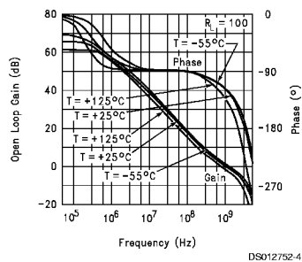
Open Loop Gain and Phase
