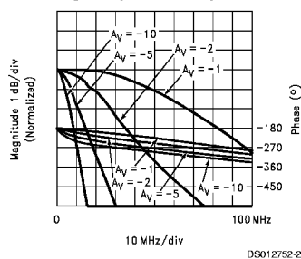
Inverting Frequency Response
