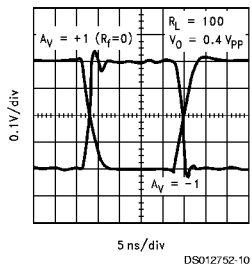
Pulse Response
