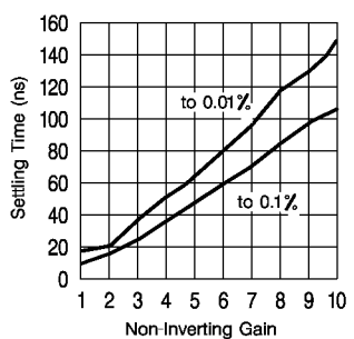
Settling Time vs. Gain
