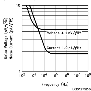
Equivalent Input Noise
