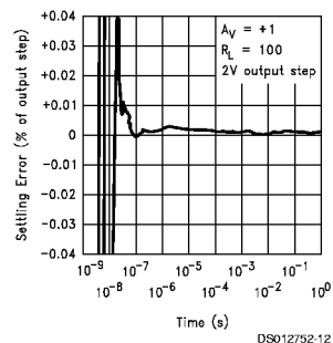
Long-Term Settling Time
