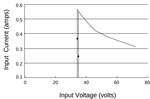
Typical Input Current Characteristics AEE04F48-197
