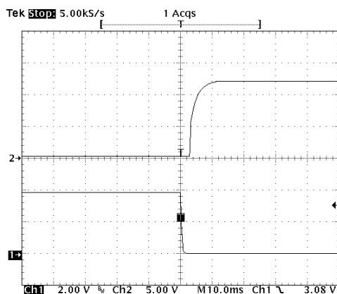
Typical Start-Up from CNT Control AEE01B48-197
