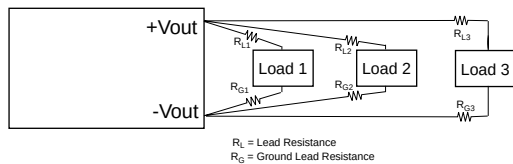
Fig.16 Radial Power Distribution
