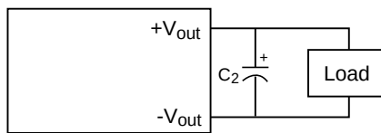
Fig.11 Output Ripple Filter
