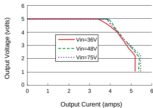
Typical Output Overcurrent Characteristics AEE03A48-197/-7/-97
