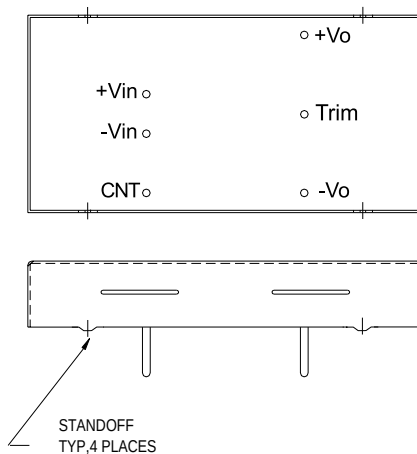
Fig.1 Pin Location
