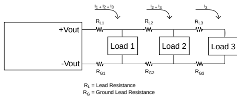
Fig.15 Parallel Power Distribution
