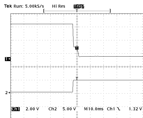
Typical Shut-down from CNT Control AEE03A48-197/-7/-97
