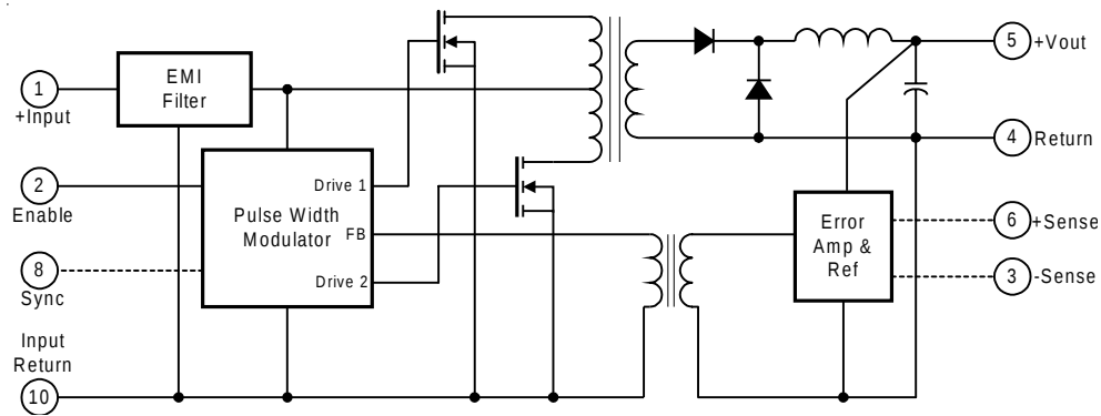
ATW28XXS Block Diagram
