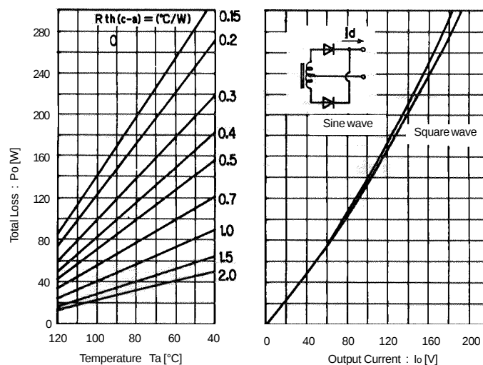
Output Current - Total Loss - Ambient Temperature
