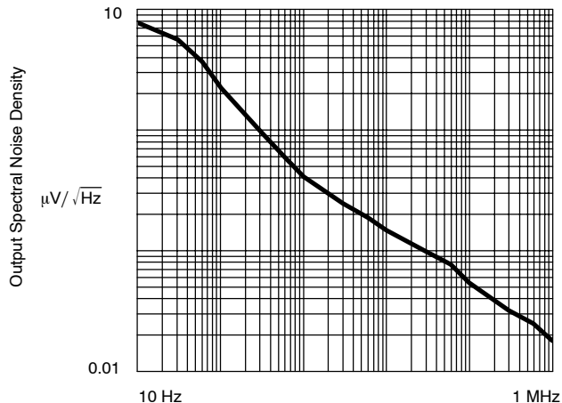
Noise Spectrum
