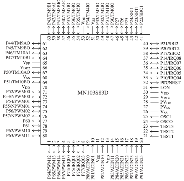
LQFP080-P-1414A *Lead-free
