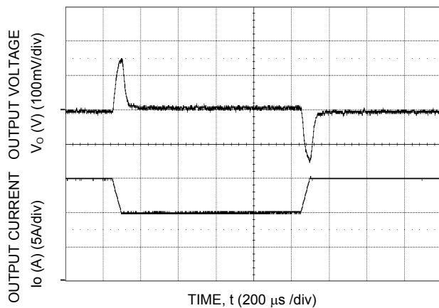
Figure 9. Transient Response to Dynamic Load Change, 0.1A/ \mu S, from 75% to 50% to 75% of full load.
