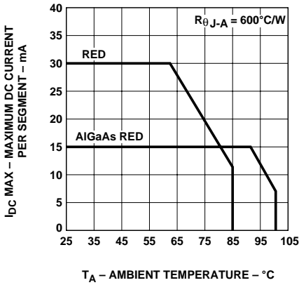
Figure 3. Maximum Allowable DC Current vs. Ambient Temperature. T_{JMAX} = 100^{\circ}C for Red and T_{JMAX} = 110^{\circ}C for AlGaAs Red.
