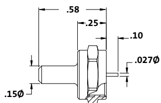
Standard 75Ω, ¼ Watt Terminator
