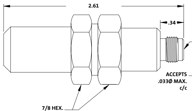
Precision Lab Grade 50Ω N Terminator
