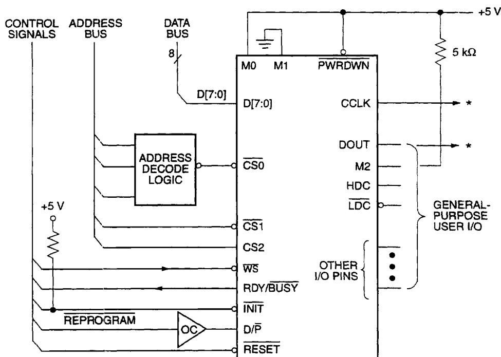
Figure 23. Peripheral Mode
