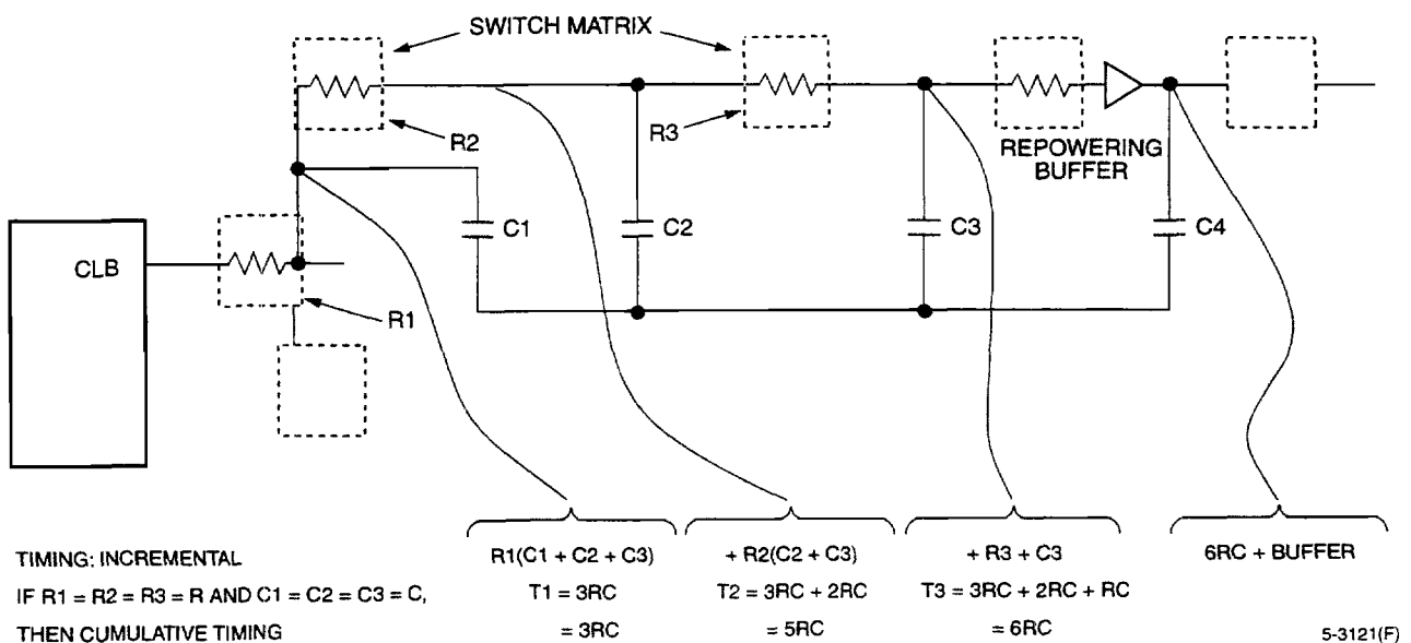
Figure 30. Interconnection Timing Example
