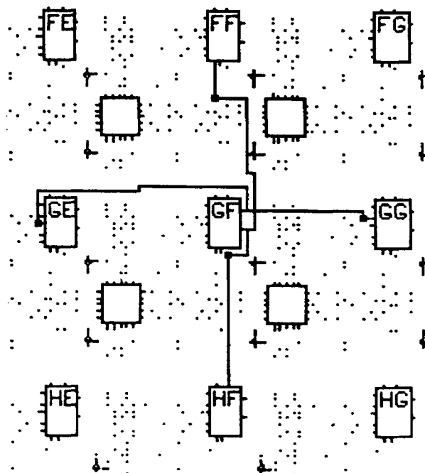
Figure 11. Direct Interconnect
