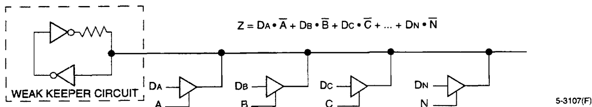
Figure 15B. 3-State Buffers Implement a Multiplexer
