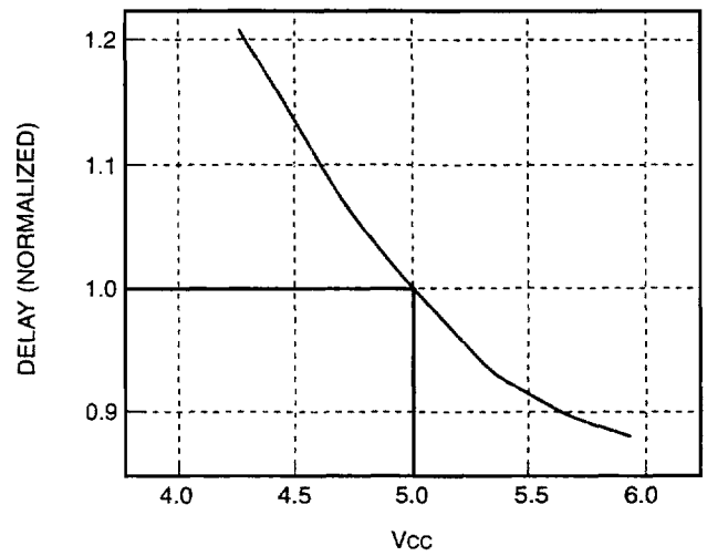
Figure 29. Speed Performance of a CMOS Device
