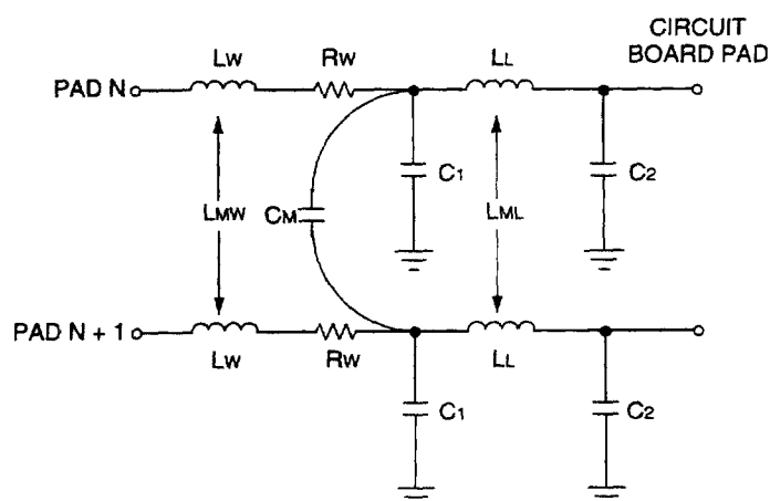
Figure 32. Package Parasitics
