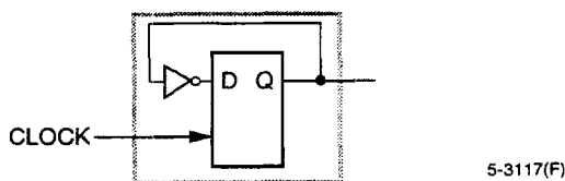
Figure 26. Toggle Flip-Flop
