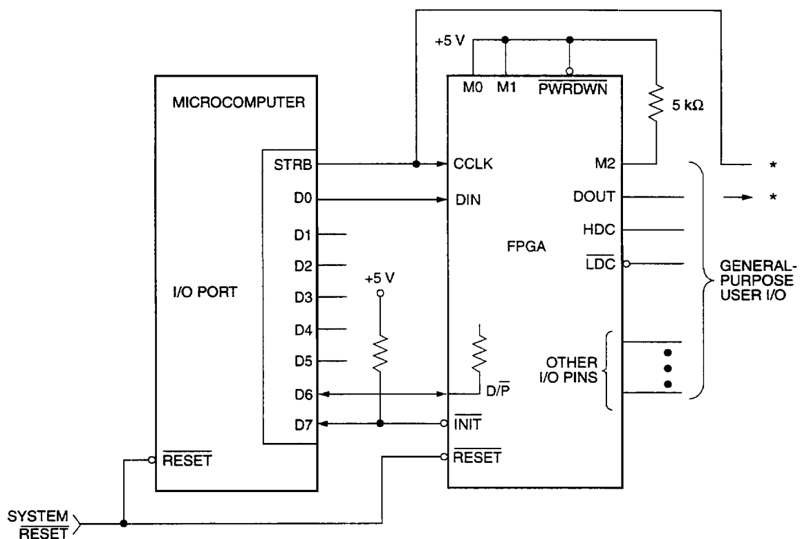
Figure 24. Slave Mode
