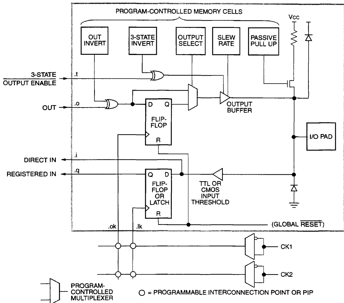
Figure 3. Input/Output Block
