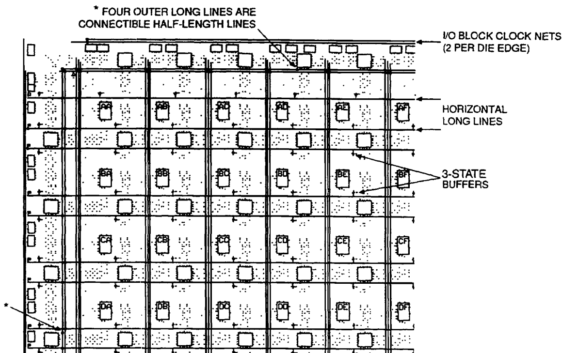
Figure 14. Programmable Interconnection of Long Lines
