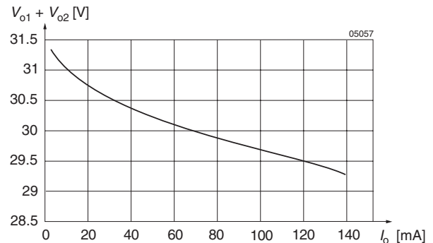
Fig. 11 V_o versus I_o (typ) of dual output units ( \pm 15 V), with 30 V load connected to V_{o+} and V_{o-} .
