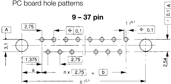
PC board hole patterns
