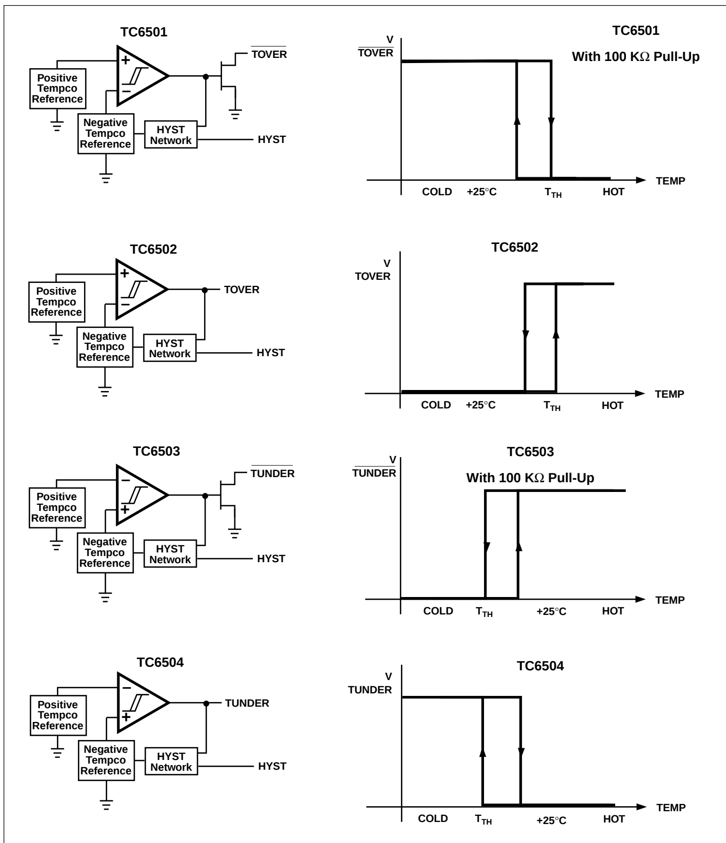
Figure 4. Functional Block Diagrams
