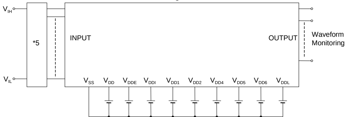
Measuring circuit 4
