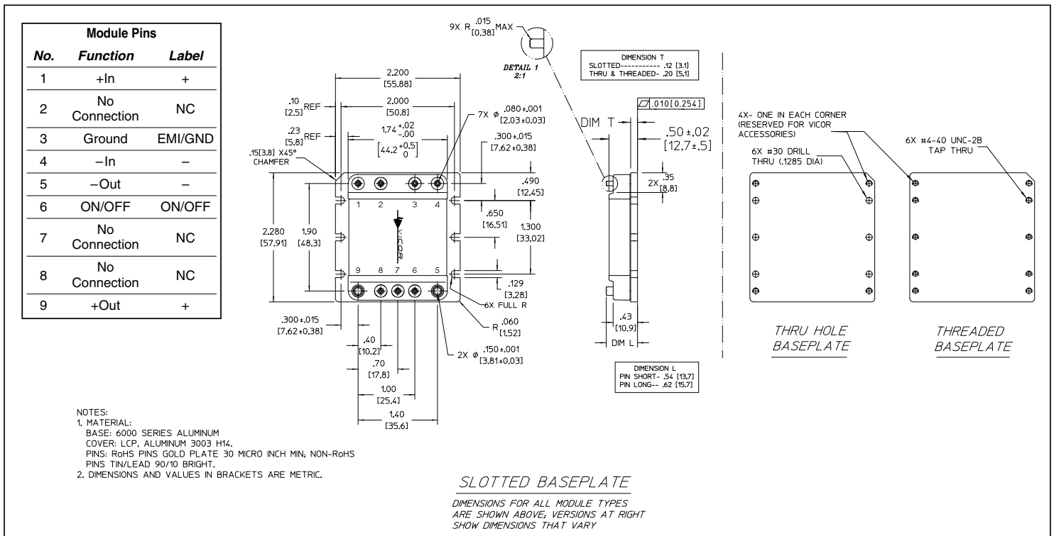
Figure 5 — Mechanical diagram
