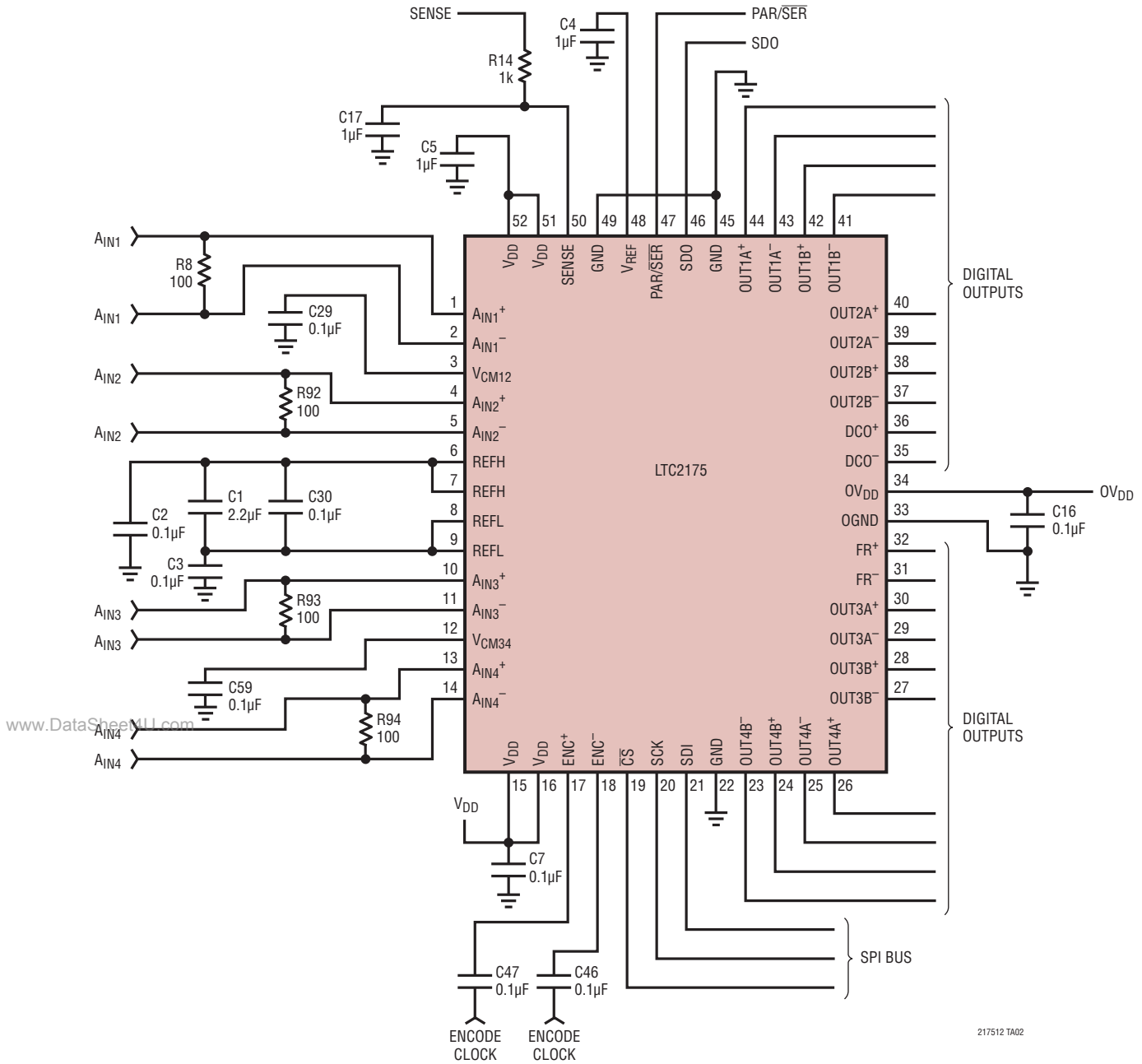
LTC2175 Schematic
