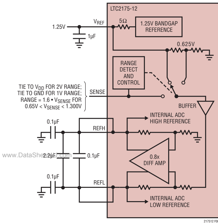
Figure 8. Reference Circuit
