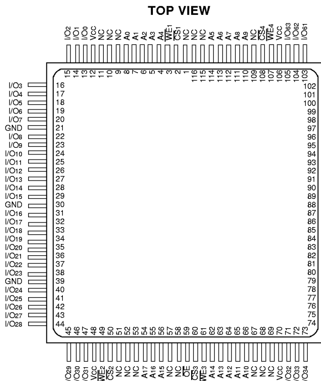
FIG. 1 PIN CONFIGURATION FOR WS256K64-XG4WX
