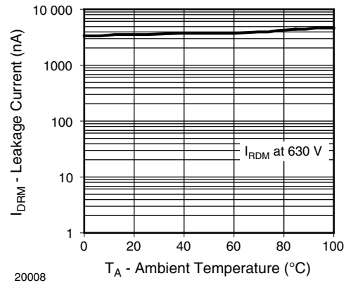
20008 Fig. 4 - Leakage Current vs. Ambient Temperature
