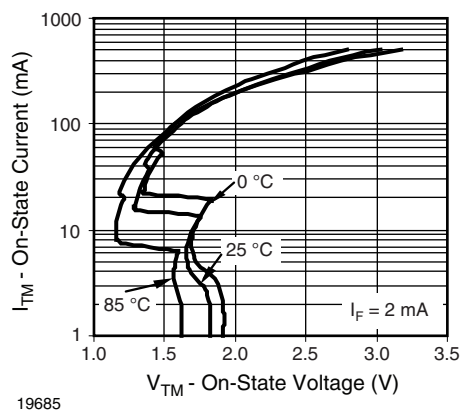
19685 Fig. 5 - On-State Current vs. On-State Voltage
