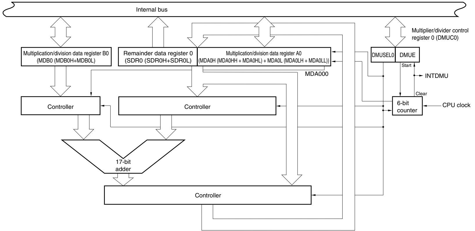
Figure 18-1. Block Diagram of Multiplier/Divider
