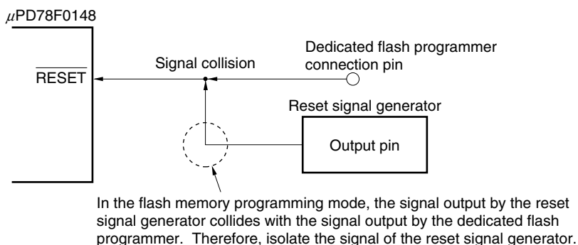
Figure 28-17. Signal Collision ( \overline{\text{RESET}} Pin)
