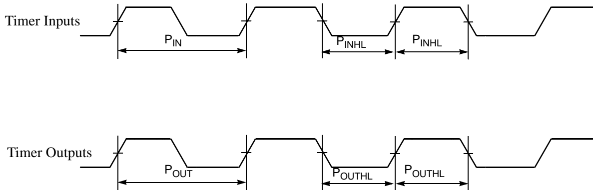
Figure 12. Timer Timing
