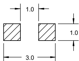
Pad Layout
