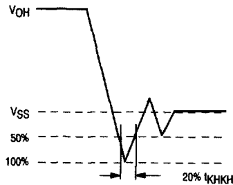
Figure 3. Undershoot Voltage
