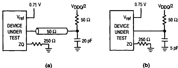
Figure 2. AC Test Loads
