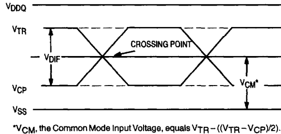
Figure 1. Differential Inputs/Common Mode Input Voltage
