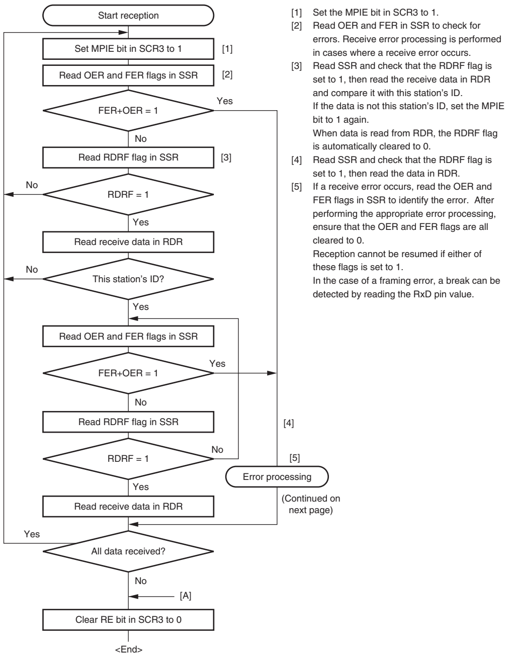
Figure 13.17 Sample Multiprocessor Serial Reception Flowchart (1)
