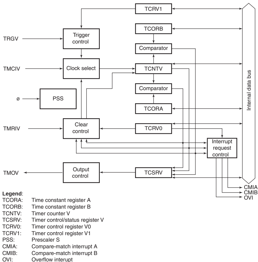
Figure 10.1 Block Diagram of Timer V
