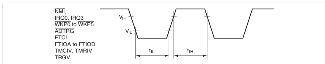
Figure 18.3 Input Timing
