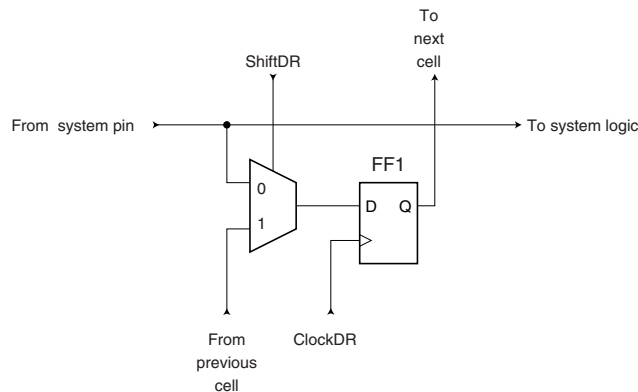
Figure 24-8. Observe-only Cell
