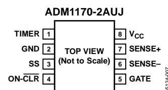
Figure 3. Pin Configuration, 2AUJ Model
