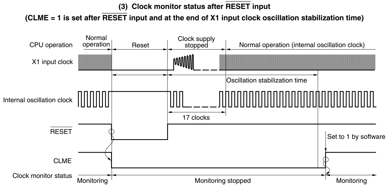
Figure 20-3. Timing of Clock Monitor (2/4)
