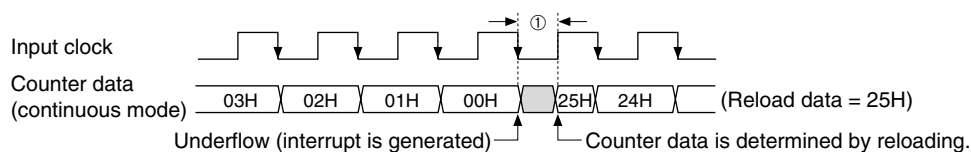
Fig. 4.10.10.2 Reload timing for programmable timer
