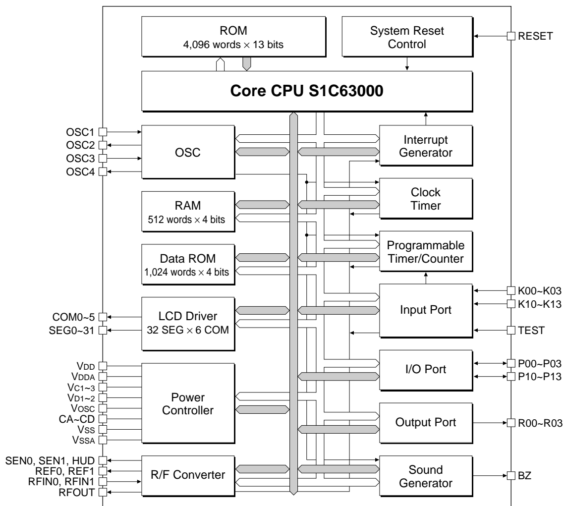
Fig. 1.2.1 Block diagram
