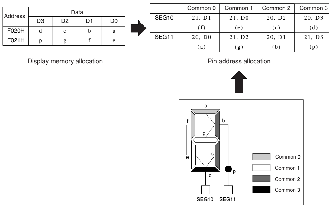
Fig. 4.8.5.1 Segment allocation
