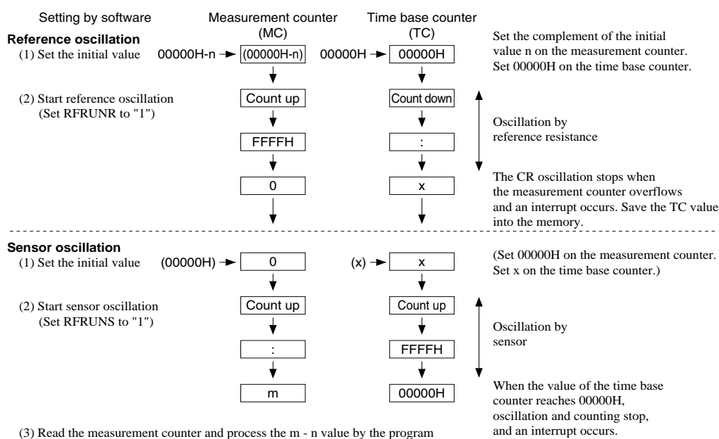
Fig. 4.12.3.3 Sequence of R/f conversion
