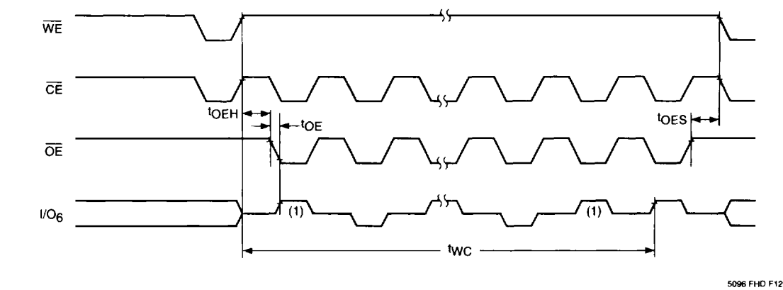
Figure 8. Toggle Bit
