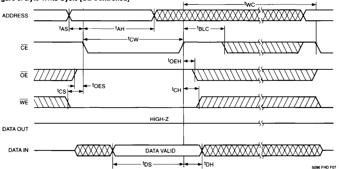
Figure 5. Byte Write Cycle [CE Controlled]
