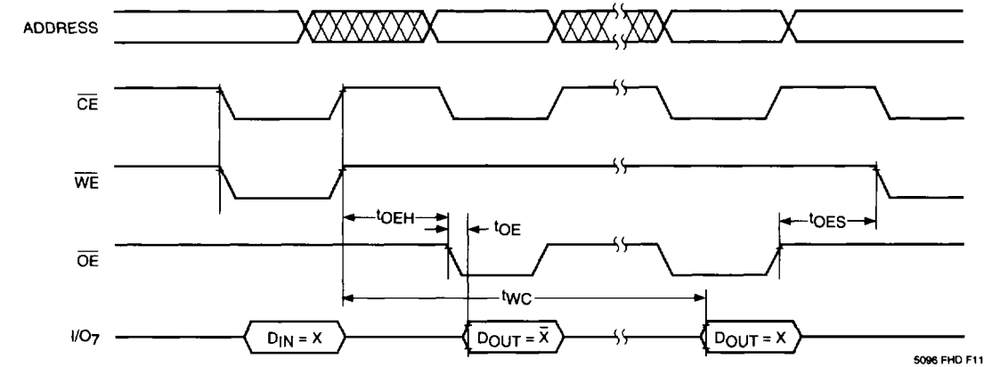
Figure 7. DATA Polling
