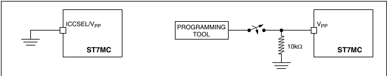
Figure 144. Two typical Applications with V PP Pin 3)
