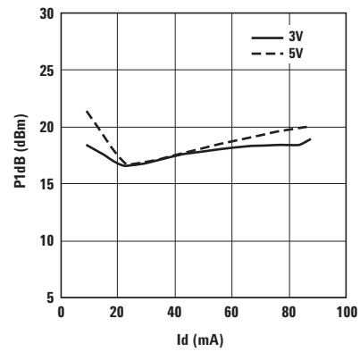
Figure 27. P1dB vs. Id (500 MHz).
