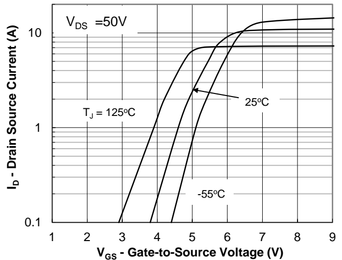
Fig.2 Transfer Characteristic
