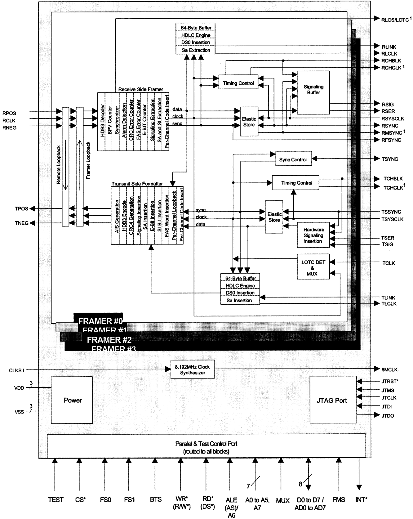
DS21Q44 ENHANCED QUAD E1 FRAMER Figure 1-1
