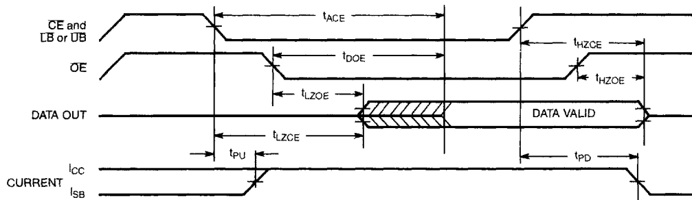
Read Cycle No.3 (Either Port) [18,20,21,22]
