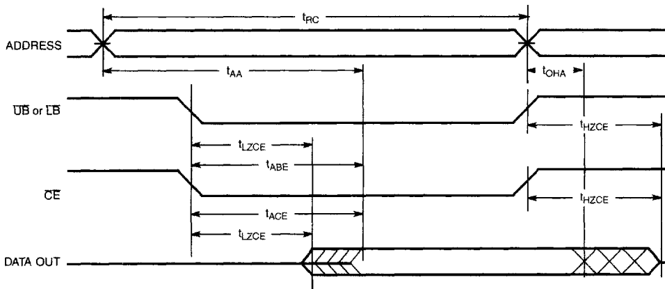
Read Cycle No.3 (Either Port) [18,20,21,22]
