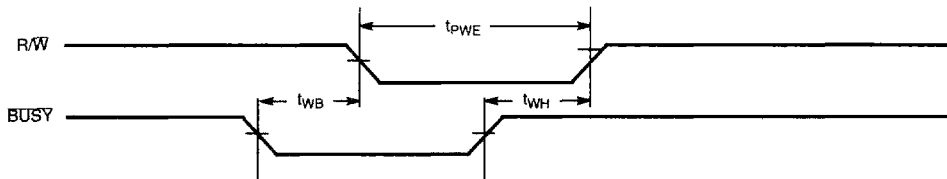
Write Timing with Busy Input (M/S=LOW)
