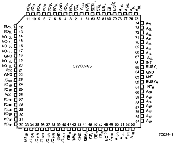
84-Pin PLCC Top View
