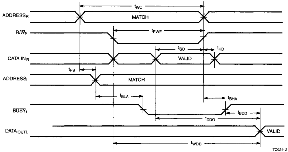
Write Timing with Busy Input (M/S=LOW)
