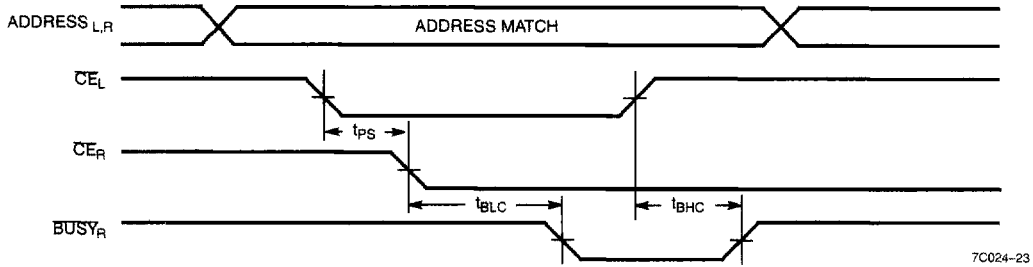
Busy Timing Diagram No.1 (CE Arbitration) [37]
