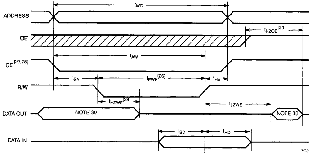
Write Cycle No. 2: CE Controlled Timing [23,24,25,31]
