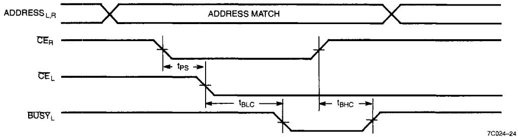
Busy Timing Diagram No.2 (Address Arbitration) [37]
