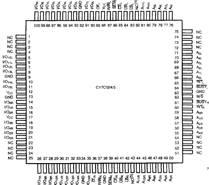
100-Pin TQFP Top View
