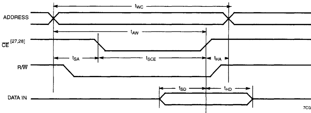
Write Cycle No. 2: CE Controlled Timing [23,24,25,31]
