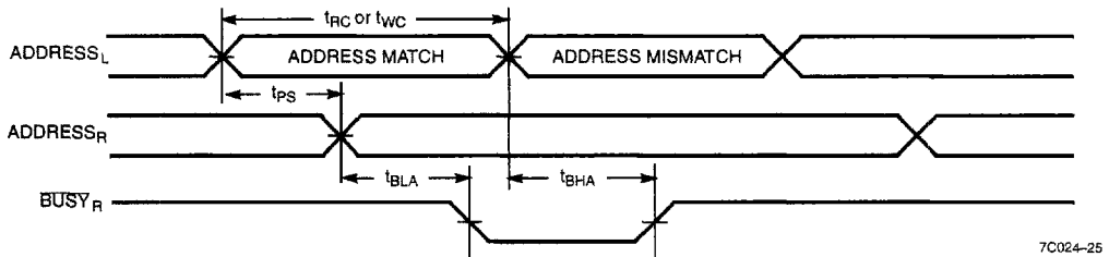
Busy Timing Diagram No.2 (Address Arbitration) [37]
