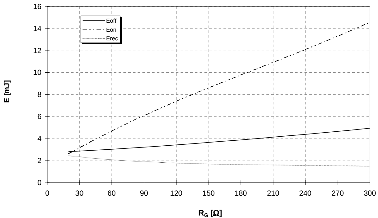
Schaltverluste (typisch) E_{on} = f(R_G) , E_{off} = f(R_G) , E_{rec} = f(R_G) Switching losses (typical) V_{GE}=15V , I_C = 25A , V_{CE} = 600V , T_J = 125^\circ C
