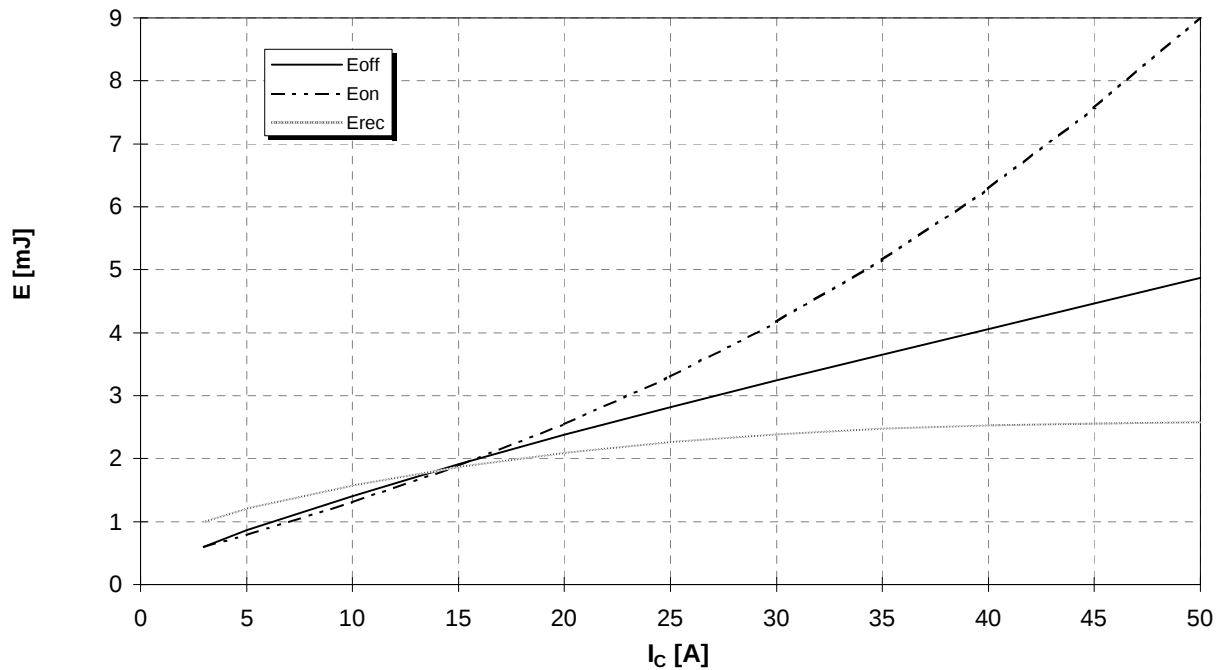
Schaltverluste (typisch) E_{on} = f(I_C) , E_{off} = f(I_C) , E_{rec} = f(I_C) Switching losses (typical) V_{GE}=15V , R_{gon} = R_{goff} = 33\ \Omega , V_{CE} = 600V , T_J = 125^\circ C
