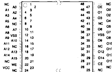
TSOP Top View Type 1
