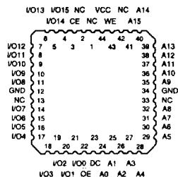
PLCC Top View
