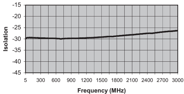
Reverse Isolation (dB)
