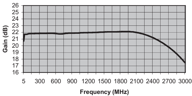
Gain (dB)
