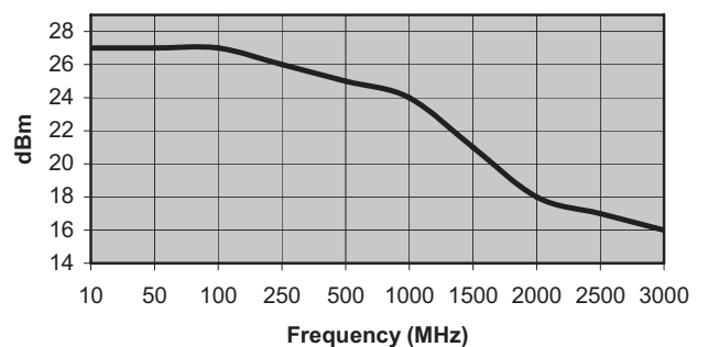
Third Order Intercept (+dBm)
